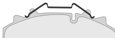
Former spring design
