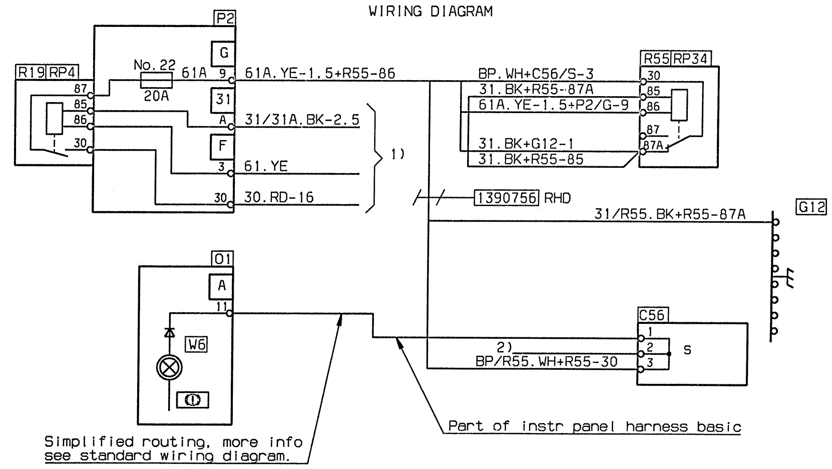
WIRING DIAGRAM
