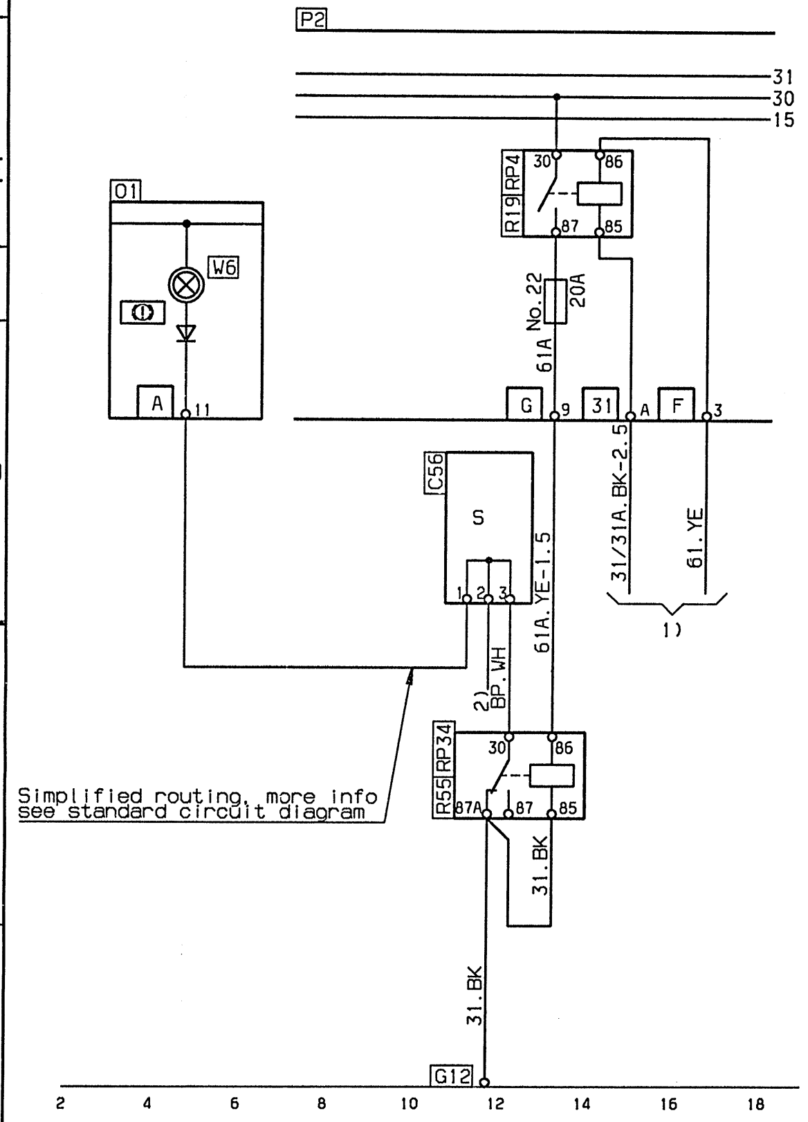
CIRCUIT DIAGRAM
