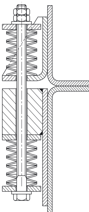
Fig. 63: Long bolts and cup springs ESC-101
