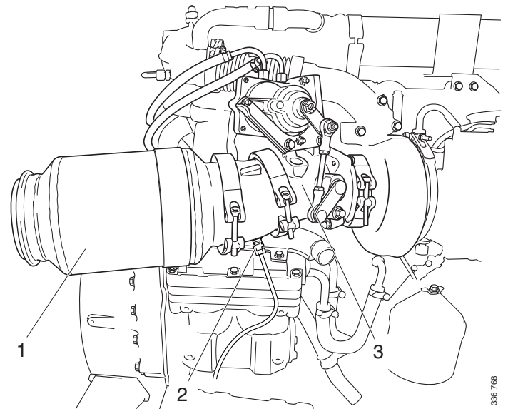
Measuring exhaust back pressure on engines with SCR system and engine-mounted oxidation catalytic converter.
