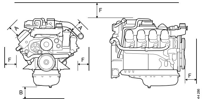
Clearances for DC16 and OC16.
