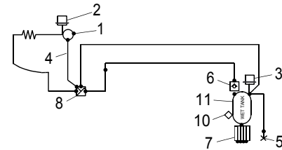
Air compressor without air dryer.
