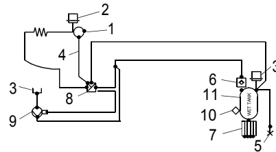
Air compressor with air dryer.
